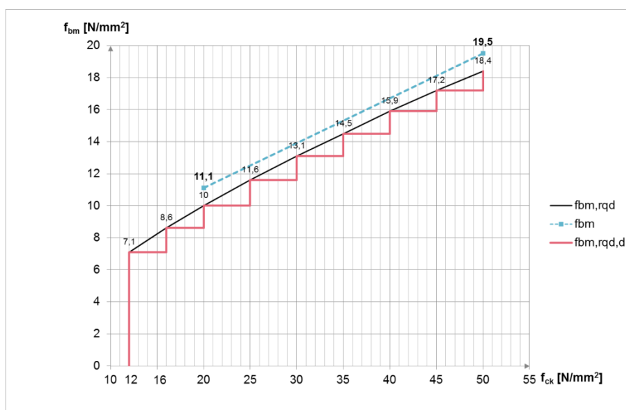
Figure 2.2 Example A: Design according to EN 1992-1-1 [1] without reduction
