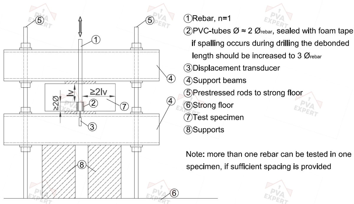
Figure 2.5 Example of pull-out test setup with displacement measurements at the unloaded end of the rebar
